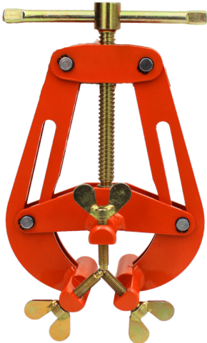
Fitting clamp 6-14" 168-355 mm
